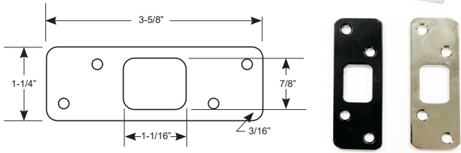
SECURITY STRIKE PLATES (REQUIRED FOR USE WITH SOME HVHZ SINGLE DOOR UNITS)
