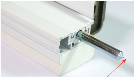
Slide bolt with machined center punch allows for precise bolt location and ease of installation.
